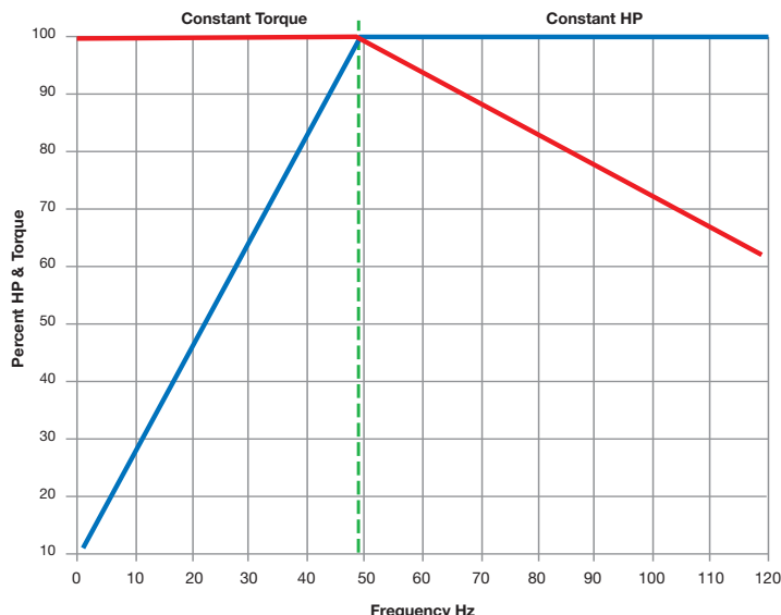
Figure (6) - Variable Frequency Drive (VFD) Speed-Torque Characteristics
