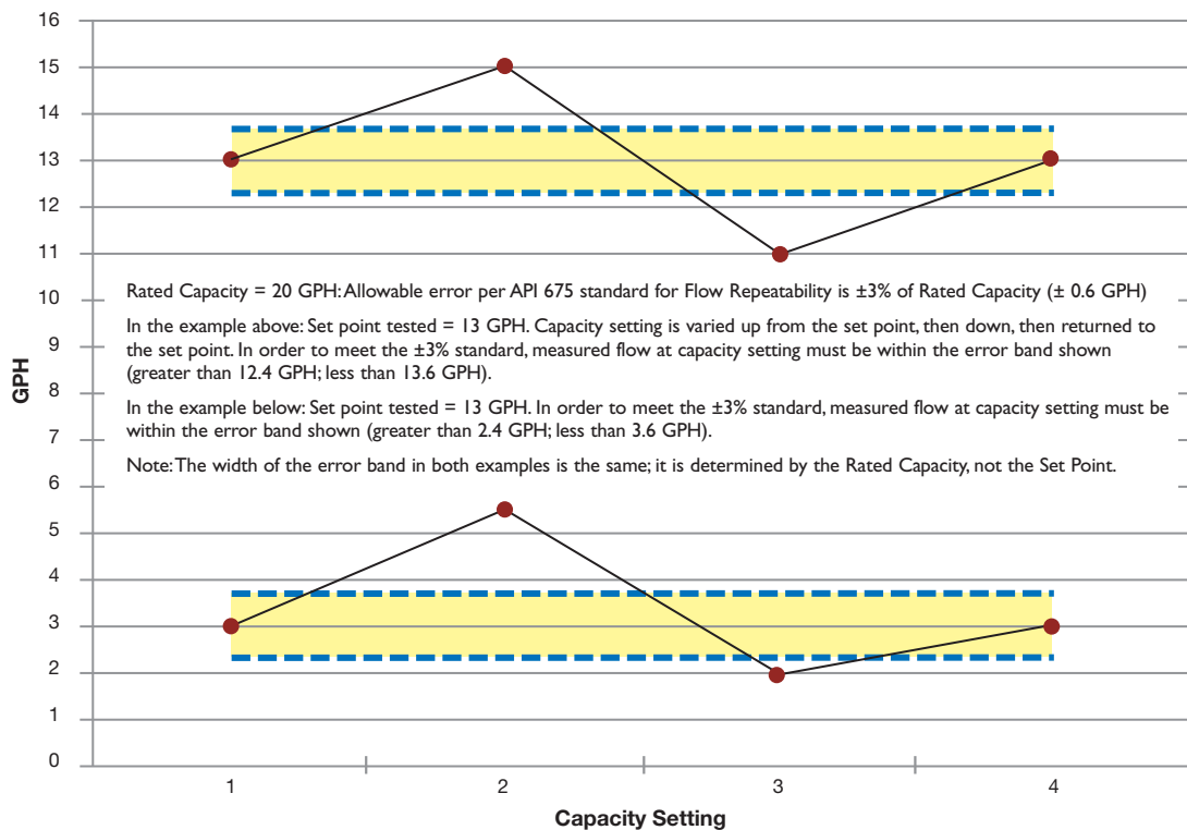
Figure (3) - Flow Repeatability
