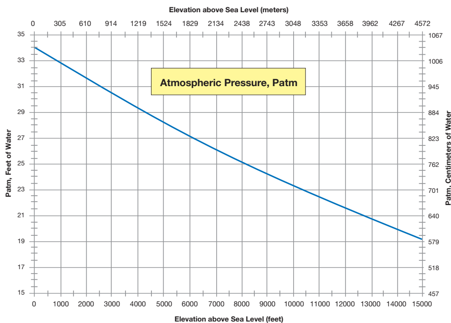
Figure (2) - Atmospheric Pressure ( P_{atm} )
