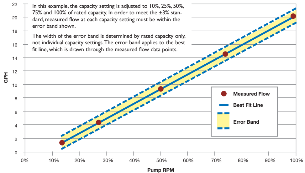
Figure (4) - Linearity
