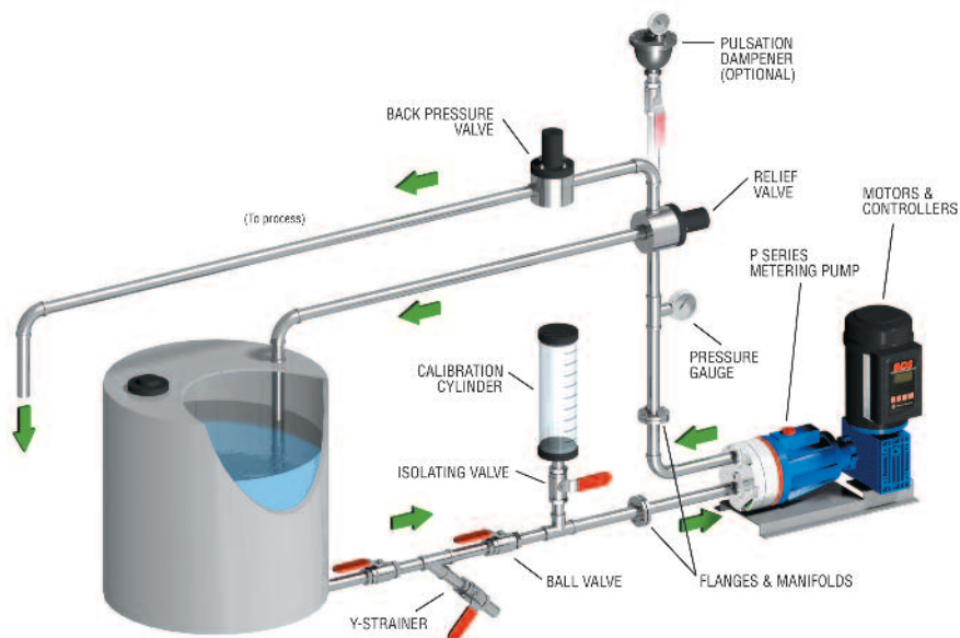
Figure (1) - Hydra-Cell Metering Solutions Sample Installation
