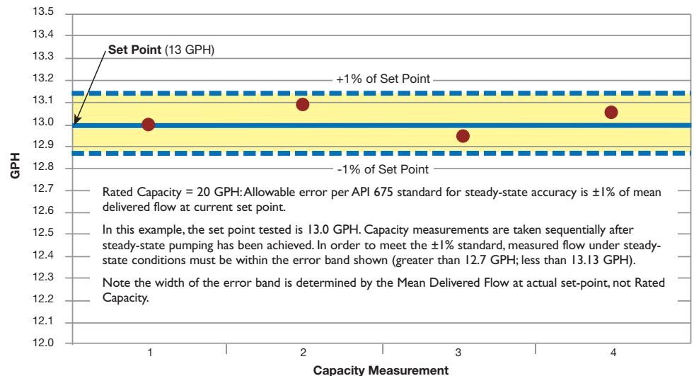
Figure (5) - Steady-State Accuracy
