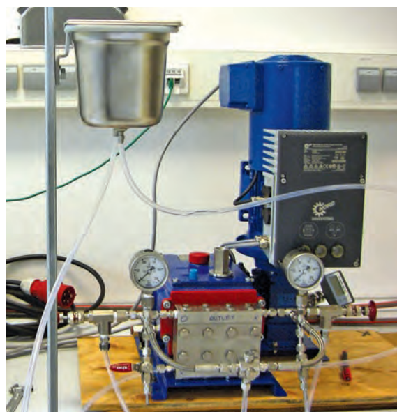
MT8 pumping aqueous and solvent-based pigment emulsions.
