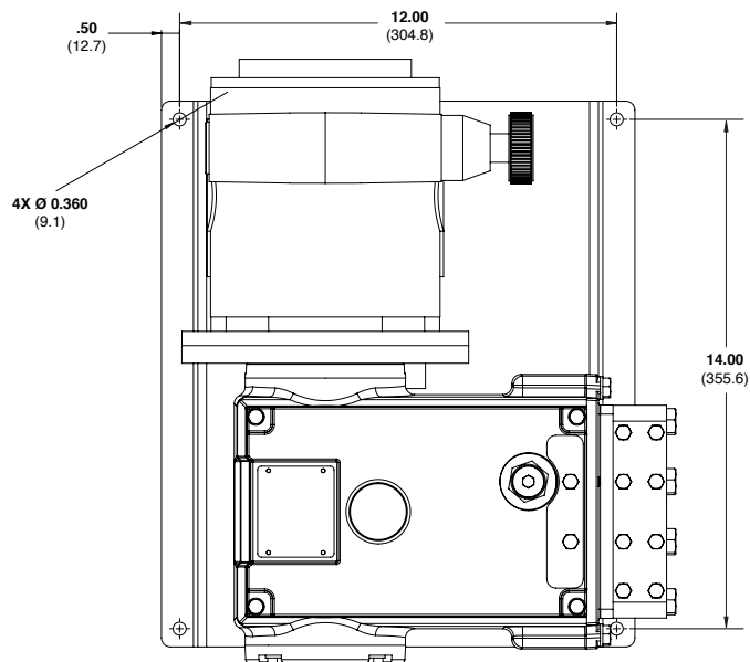
Metallic Pump Heads with Manual Adjustment Inches (mm)
