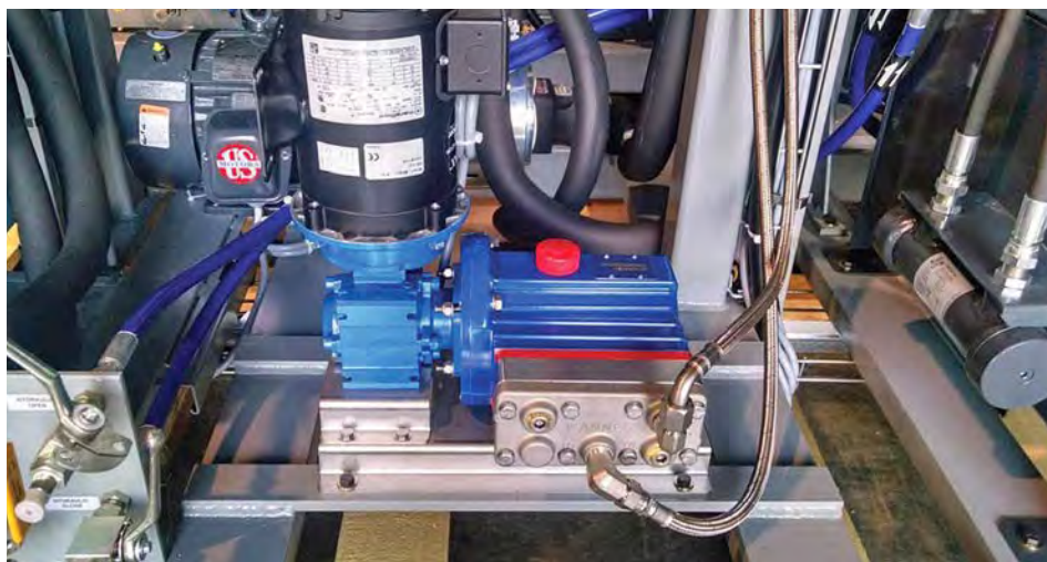
A P200 replaced an external gear pump to deliver a catalyst for polyurethane foam production and doubled volumetric efficiency.
