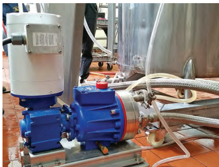
P400 used for spray drying of non-lubricating as well as viscous flavor additives in the food processing industry.
