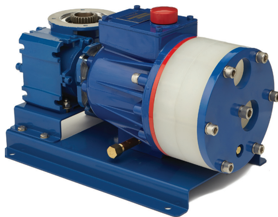
P400 with Polypropylene pump head
