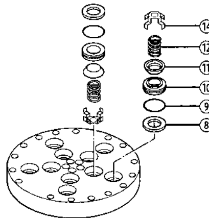
Valve Assemblies with metal spring retainers
